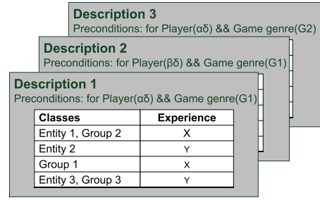
Figure 4: Example of semantic gameplay descriptions, with notation consistent with Fig. 2
