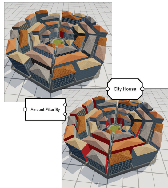
FIGURE 9: Example of the need to enforce execution scopes. If all the façades are collected without differentiation, only one facade of the whole building set would be selected, instead of one per building.
