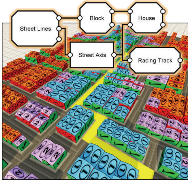
FIGURE 1: Our graph-based approach introduces context-awareness verifications which can be applied at any step of the generation process. Here, we perform visibility calculations to determine which façades are visible (marked in green) from a highlighted street (marked in yellow) and which are not (marked in red). We also calculate the minimum distance of each house towards that same street and decide on a level of detail (1, 2, or 3, as marked on the roofs) based on the distance. For applications focused on a main path, for example, racing games, this information could be used to guide the procedural content generation and include budget considerations in the construction of the virtual world.
