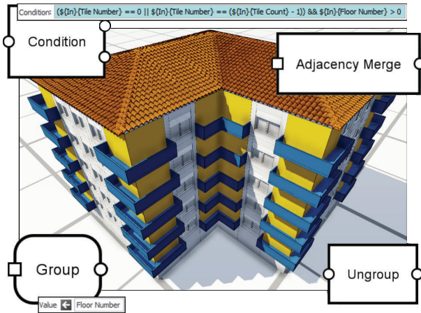
FIGURE 6: Building featuring balconies that stretch across façade corners, an example that cannot be naturally achieved using shape grammars.
