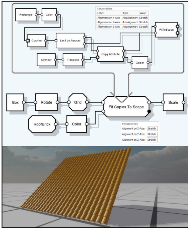
FIGURE 5: Encapsulation of a graph that extends the “fit-to-scope” operation to lists. The thick-line ports indicate the gates of the graph, which are mapped to the encapsulated node’s ports. Graph parameters are also mapped to the node’s parameters. The supergraph uses this encapsulated graph to easily copy and fit a brick rooftop into each cell of a rectangular grid (both brick and grid are also encapsulations). The result is a detailed roof surface.
