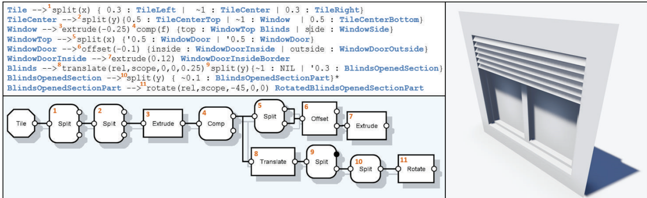
FIGURE 2: Window example modeled using a CGA shape grammar formulation (upper left; loosely based on [3] and [38]) and our procedural content graphs (lower left), each rule operation corresponding to a node with a matching number. The visual nature of our approach makes the flow of data easier to follow and does not require the user to come up with rule symbols (highlighted in blue) or geometric labels [6, 7], which generally make management difficult and error-prone.
