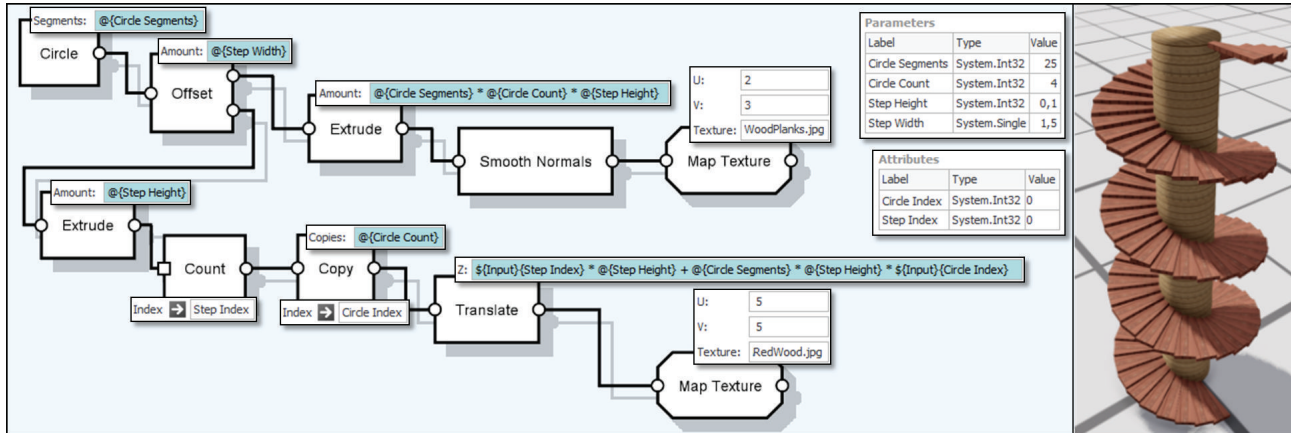
FIGURE 4: Construction of a stairway using attributes. An offset is applied to a circle to extrude polygonal steps. These are counted and assigned an index attribute. The steps are copied and an additional copy index is assigned. The steps' translation is steered via these attributes. The boxes above the nodes indicate the assigned fixed values (in white) or expressions (in blue). The notation \text{\$[parameter label]} is used to refer to graph parameters, while \text{\$[port label]\{attribute label\}} is used to refer to an attribute of an entity coming from a certain node port. The boxes with arrows under the nodes indicate attribute mapping.
