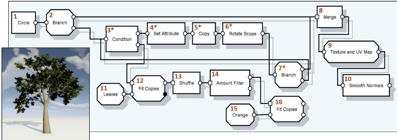
FIGURE 3: Orange fruit tree generated using a cyclic PCGR. The node numbering indicates the topological ordering of the nodes and the ones marked with an asterisk are bound to be executed multiple times, as they are found within a loop.
