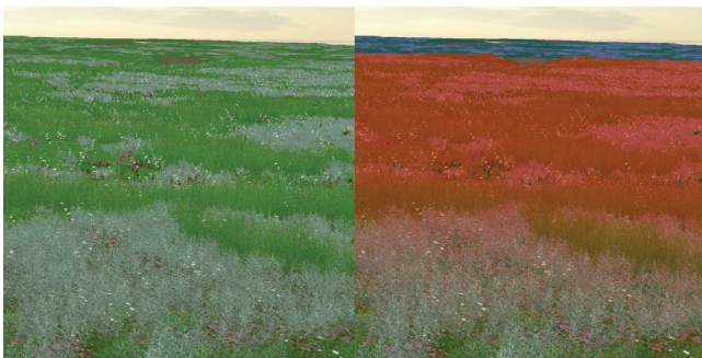
Figure 17: Transition of the various LODs in the virtual Paulinapolder. Green are the regular plant models, red are the billboards, blue is the terrain color map.
