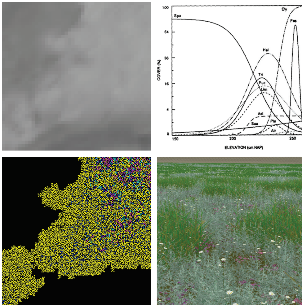
Figure 4: A visual overview of our approach starting with the various input data (top), such as landscape maps and statistical data [de Leeuw et al. 1994]. Next, from this data we derive the plant distribution in the vegetation model (bottom left), where each point is associated to plant species. Finally, from this plant distribution we derive the detailed 3D visualization model, suitable for rendering in the browser (bottom right).
