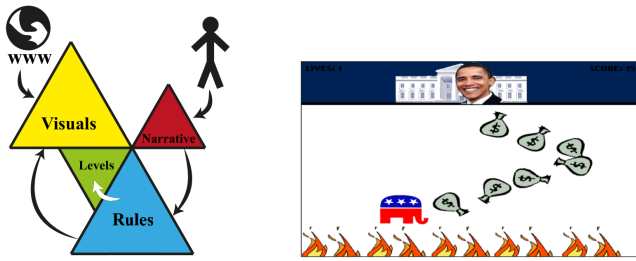
Fig. 8: Facet orchestration in Game-O-Matic, where a human-authored micro-rhetoric (small-scale narrative) informs which game objects and rules exist in the gameworld; game objects get their visuals from online sources through a search query based on the micro-rhetoric. In-game screenshot is from [89].
